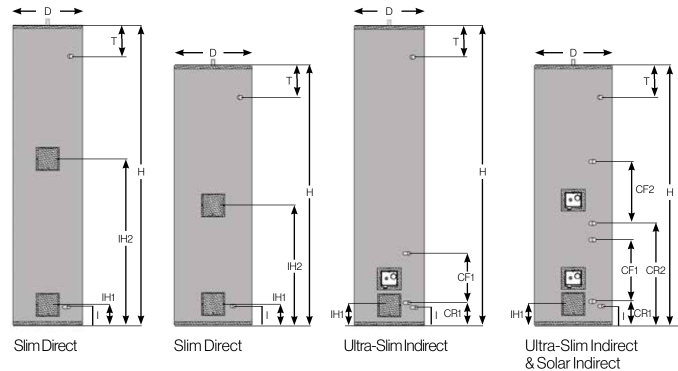
Slim Direct with external expansion
